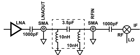
\Pi COMPONENTS SHOWN ARE FOR 900MHz RF A “T” FILTER CAN ELIMINATE THE 1000pF COUPLING CAPACITORS
